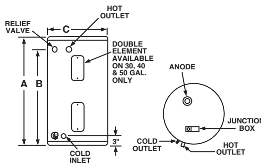
WATER CONNECTIONS ALL 3/4" N.P.T.
