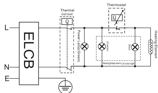
Diagram 7 Wiring diagram
