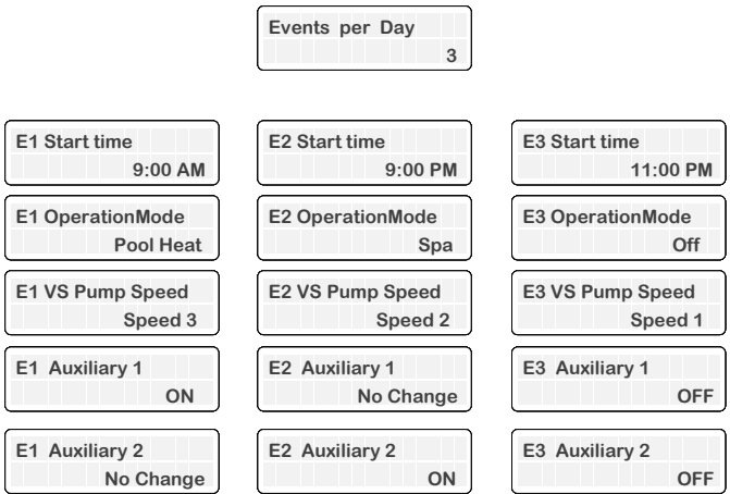
Figure 55. Events Programming Option
