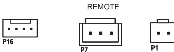
Figure 59. Remote Wiring Connector
