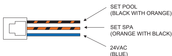
Figure 61. 3-Wire Remote Harness
