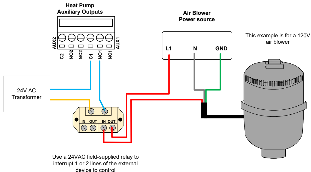
Figure 150. Example 2: Air Blower Wiring
