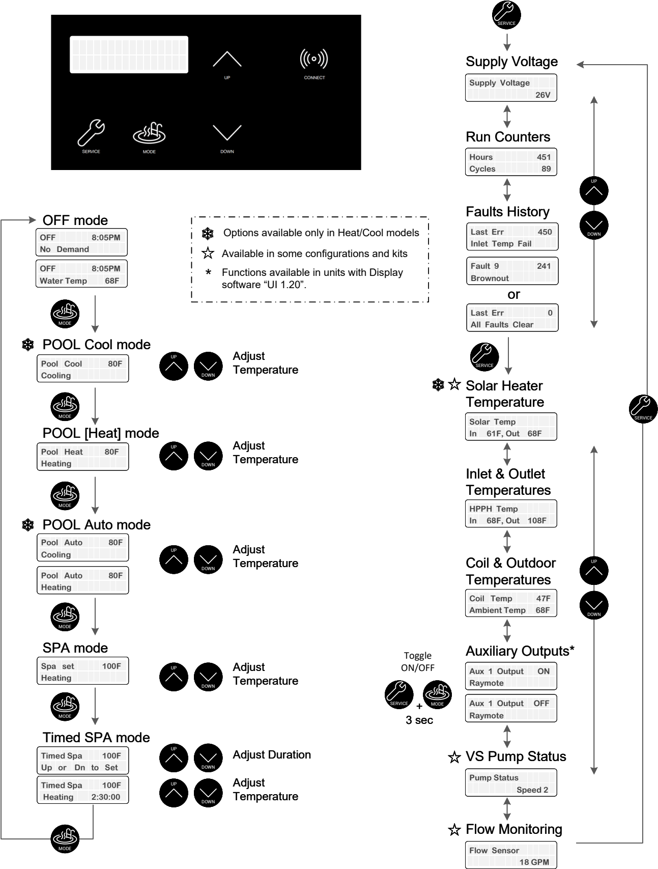
Figure 24. Operation and Service Screen
