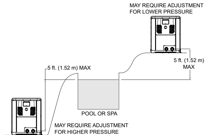
Figure 58. Pressure Switch Adjustment Requirements
