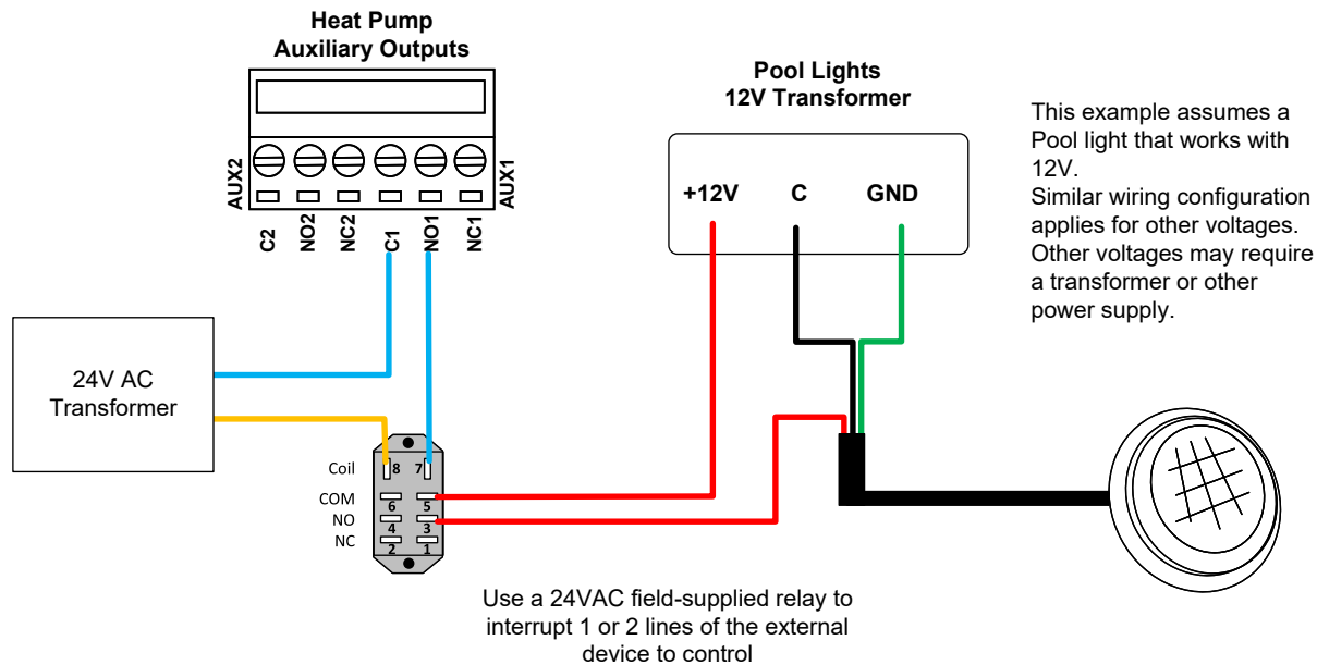
Figure 149. Example 1: Pool Light Wiring
