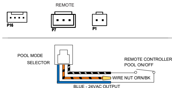
Figure 64. 2-Wire Remote Harness Installation
