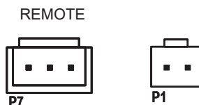
Figure 32. Remote Wiring Connector
