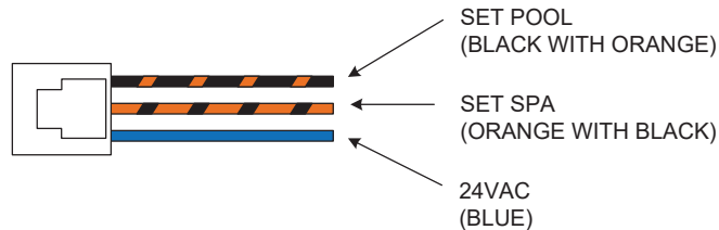
Figure 34. 3-Wire Remote Harness
