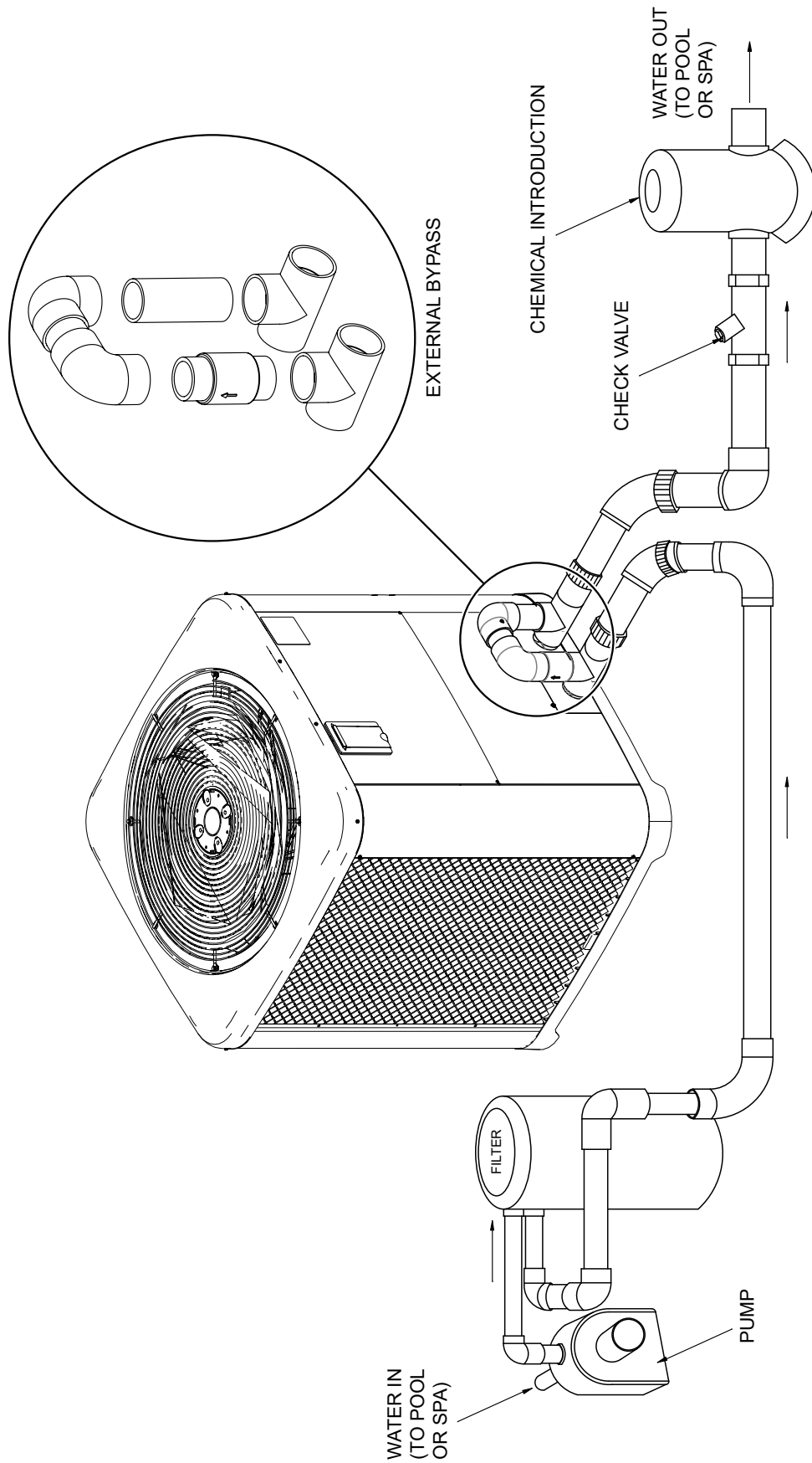
Figure 41. Plumbing Schematic – External Bypass (Plumb the heater AFTER the filter and before any chlorinators.)
