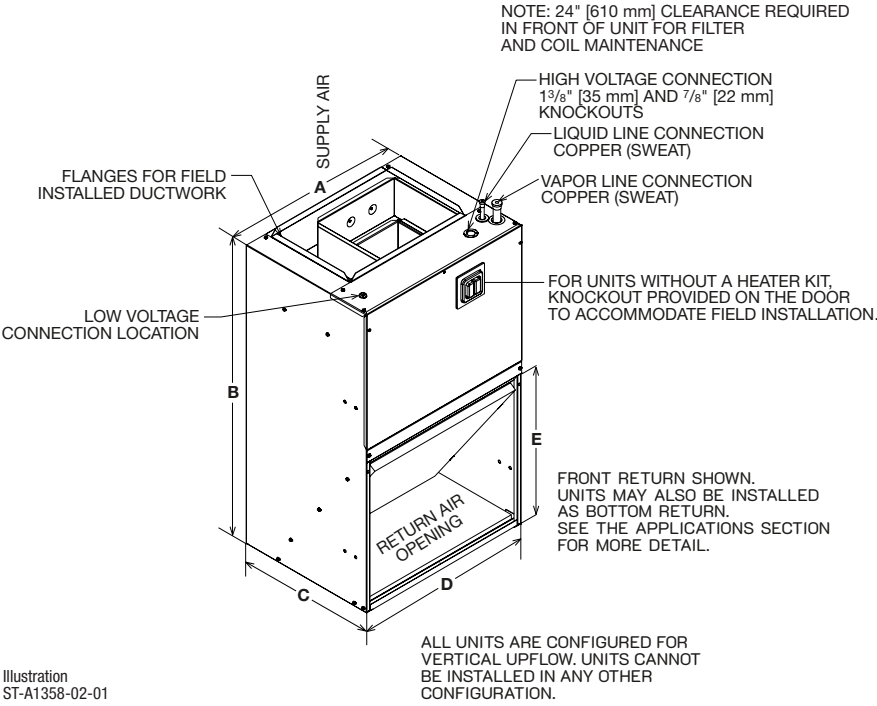
Return Air Opening Dimensions
