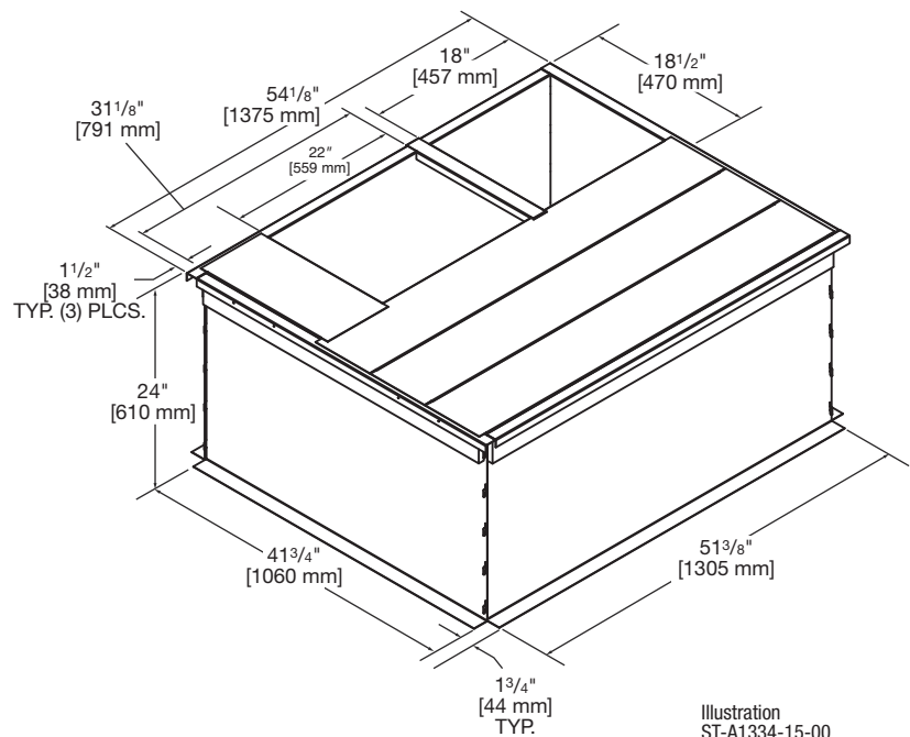
RXSG-AXA24 (24" [610 mm] Height)
