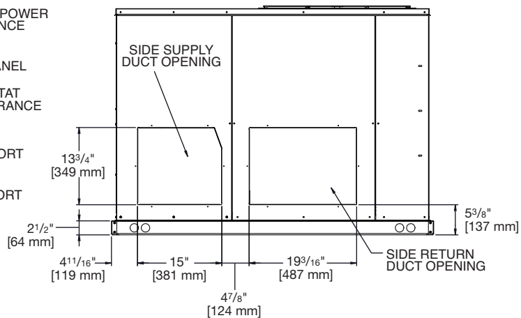
REAR VIEW
