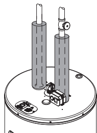
Typical vertical piping arrangement (Shutoff Valve Optional)
