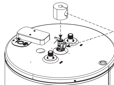
Typical top connection arrangement (Optional Shutoff Valve Not Shown)
