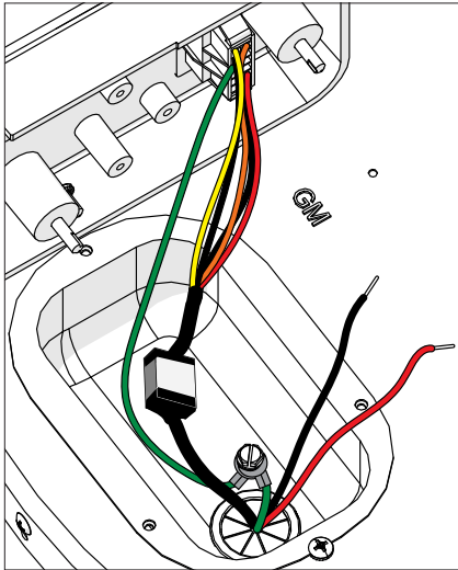
Water heater junction box.
