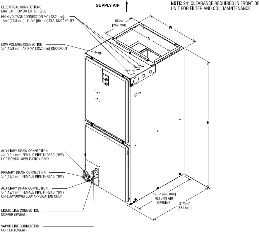
Return Air Opening Dimensions
