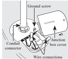
Water heater junction box.
