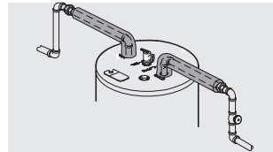
Typical horizontal piping arrangement
