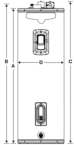
WATER CONNECTIONS ALL 3/4" N.P.T.
