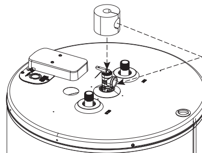
Typical top connection arrangement
