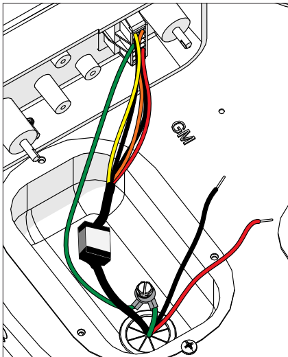
Water heater junction box.
