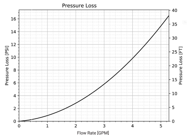
Water heater pressure drop – L-Series RMTGH-L199i
