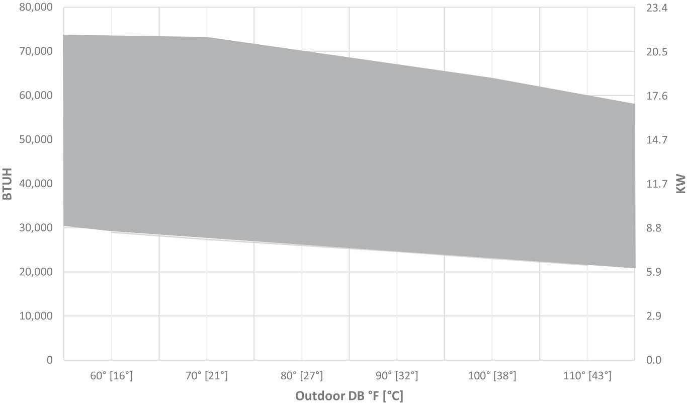
(-)P18AZ60 Cooling Capacity Ranges
