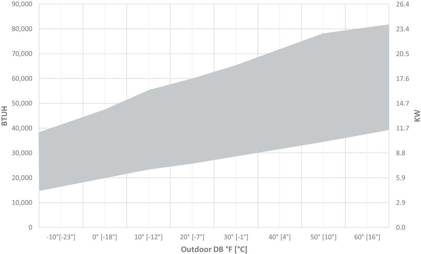
(-)P18AZ60 Heating Capacity Ranges
