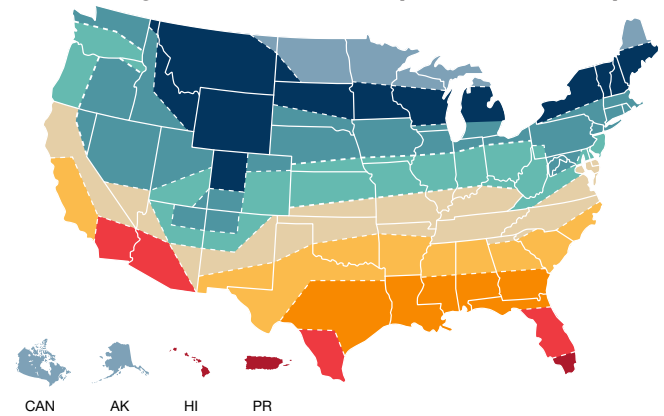
U.S. Average Ground Water Temperature Zone Map
